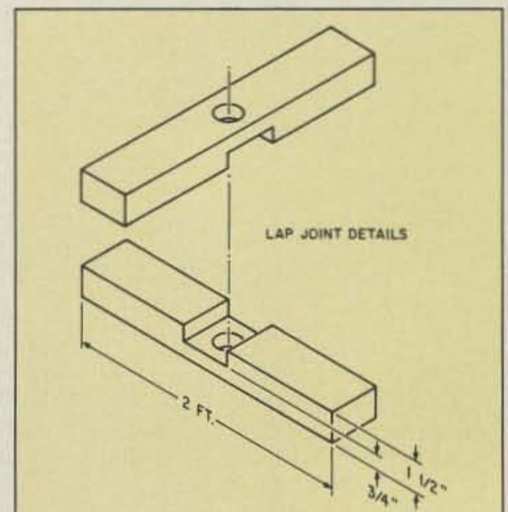
Figure 2. Lap joint for assembly of the X-mount.
